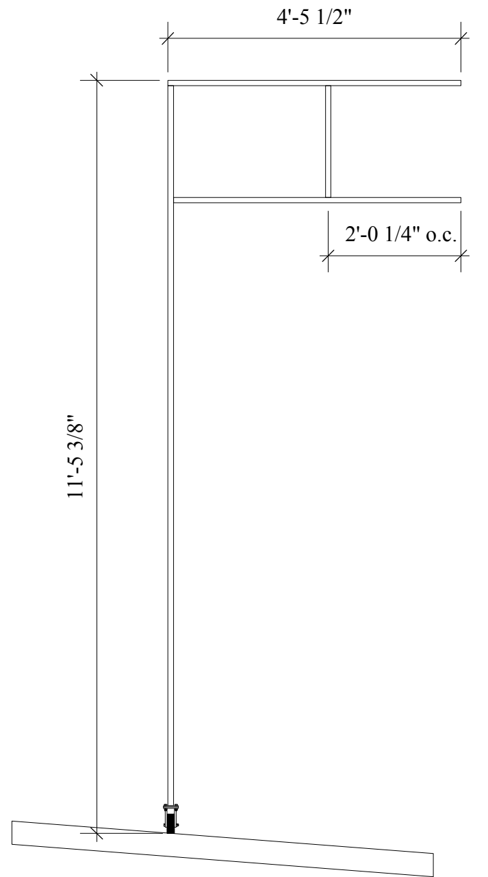
SIDE VIEW U.S. ARCH UNIT FRAME R&R STAGE RT ARCH UNIT FRAME
