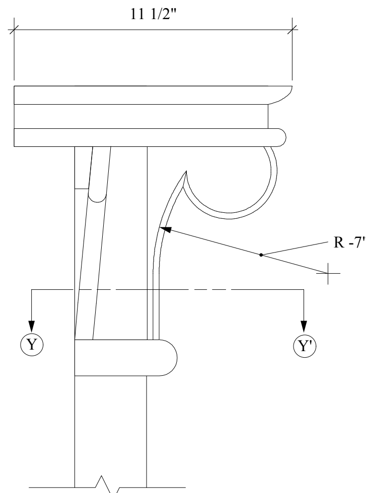
SIDE VIEW OF CORNER CAPITAL SCALE: 3"=1'-0"
