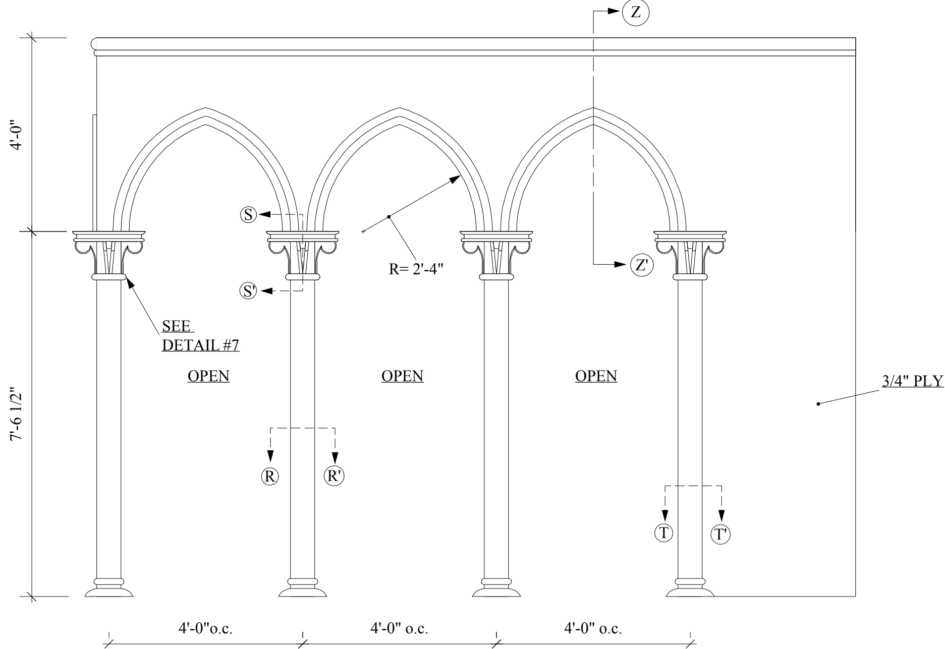
UPSTAGE LEFT ARCH UNIT R&R FOR STAGE RT ARCH UNIT
